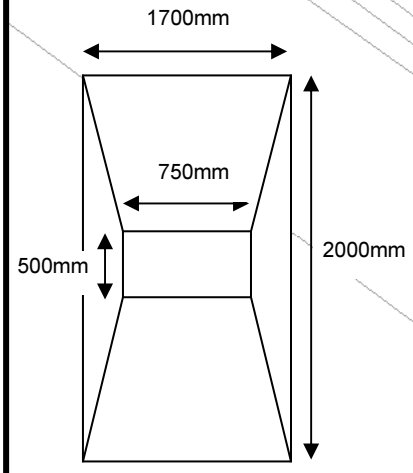
Speed Cushion Dimensions
